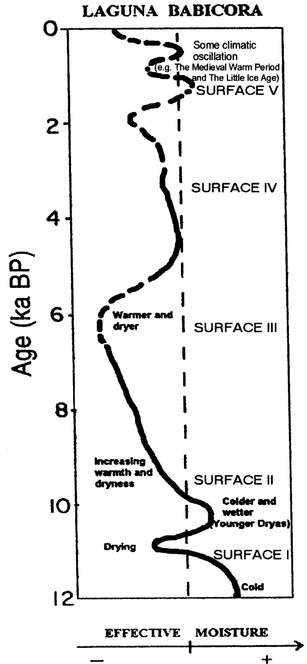
Fig. 10. Paleoclimatic correlation between the alluvial fan surfaces studied in this work, and the general effective moisture curve established for the Laguna de Babicora from the Late Wisconsinian to late Holocene. The dashed extension of the curve represents interpolated data from previous studies (Ortega-Ramírez et al. , 1998, 2000).
