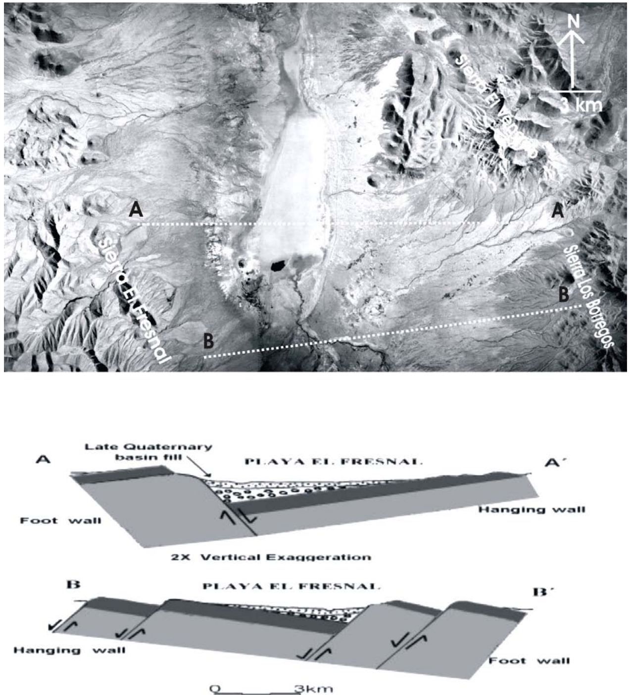
Fig. 5. Airphoto view of alluvial fans and geomorphologic features of the El Fresnal Playa Lake. Dotted lines A-A' and B-B' are the traces of the cross-sections shown in figure. Note that the foot-wall catchments are shorter and steeper than those in the hanging-wall.
