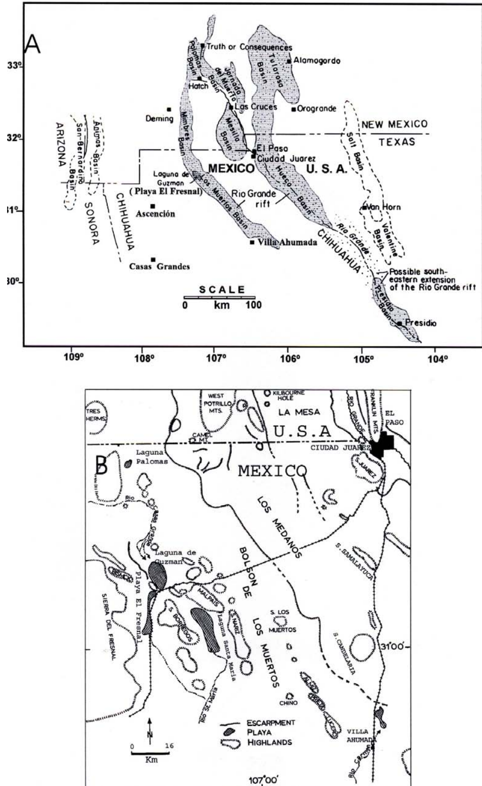
Fig. 2. (A) Bolsons in the southern Río Grande Rift of Texas and New Mexico, United States, and of Chihuahua, Mexico (Map modified from Stuart and Willingham, 1984); (B) Northwestern Chihuahua showing the general area of pluvial Lake Palomas and the playa lakes: Laguna de Guzmán, Playa El Fresnal and Laguna Santa María: (Map modified from Reeves, 1969).
