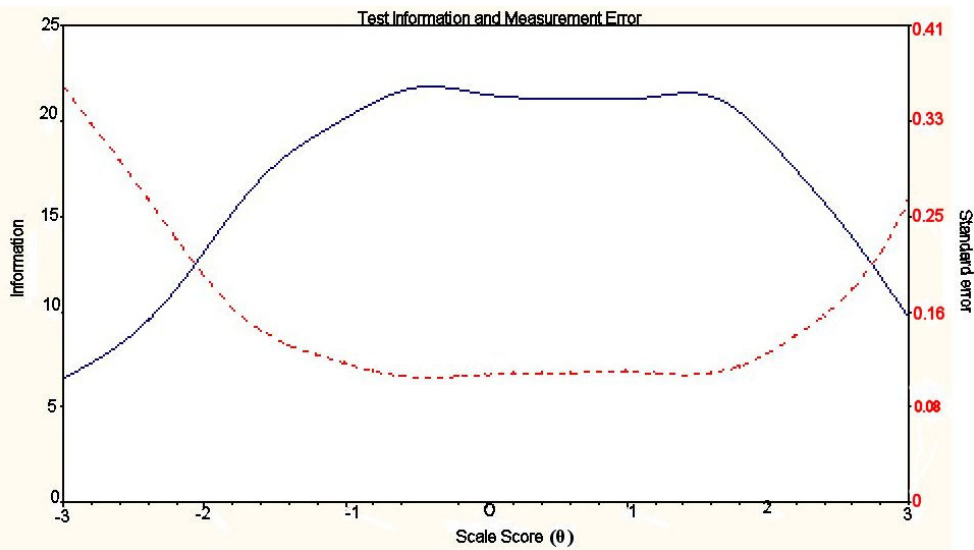
Figure 2 Total information across the construct for Ab-A. Test information curve - solid line; Standard error curve - dotted line.
