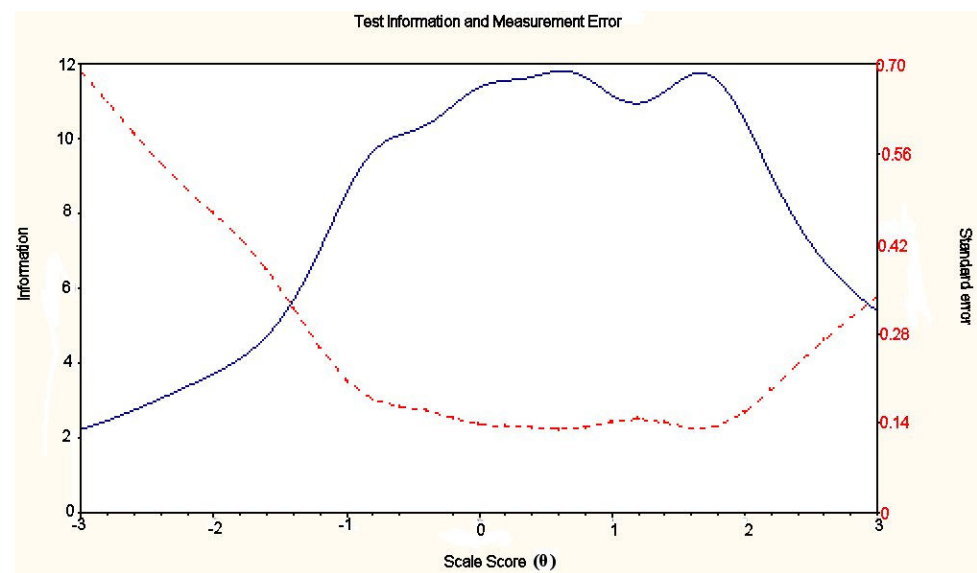
Figure 4 Total information across the construct for Ab-P. Test information curve - solid line; Standard error curve - dotted line.
