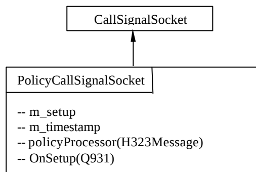
Figure 25. CallSignalSocket Class
