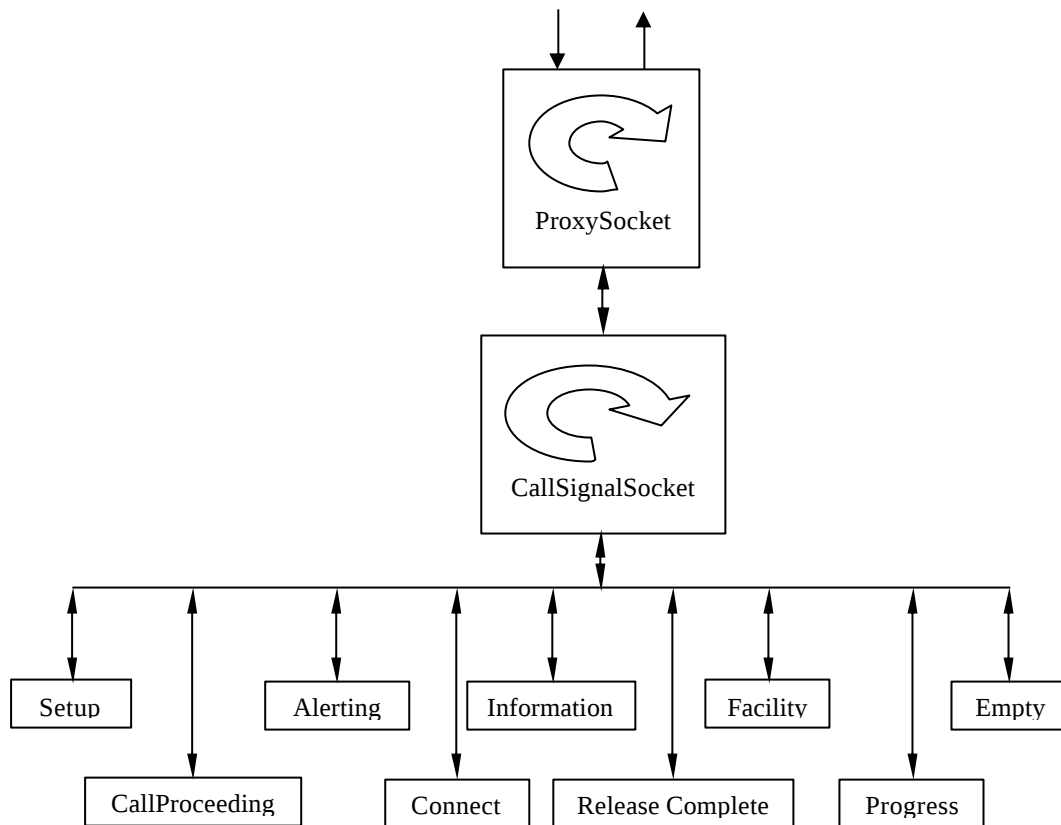
Figure 25. CallSignalSocket Class
