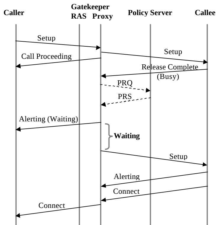
Figure 10. Waiting-on-Busy policy
