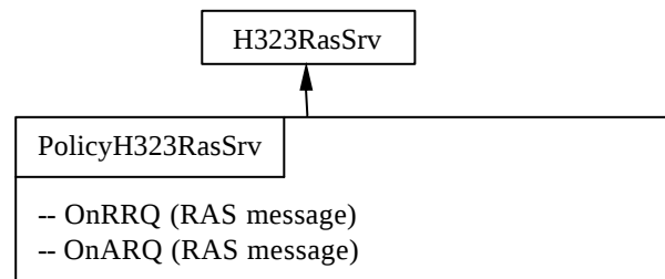
Figure 26. PolicyCallSignalSocket Class
