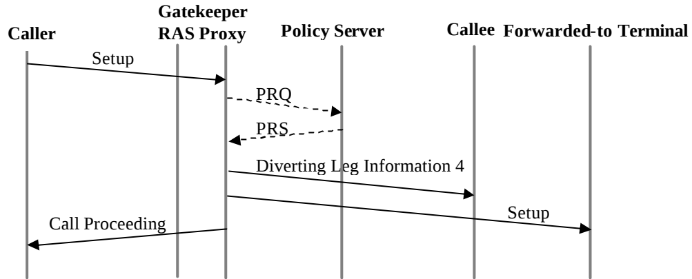
Figure 8. Forward-Always Policy
