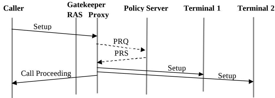
Figure 13. Forking Policy
